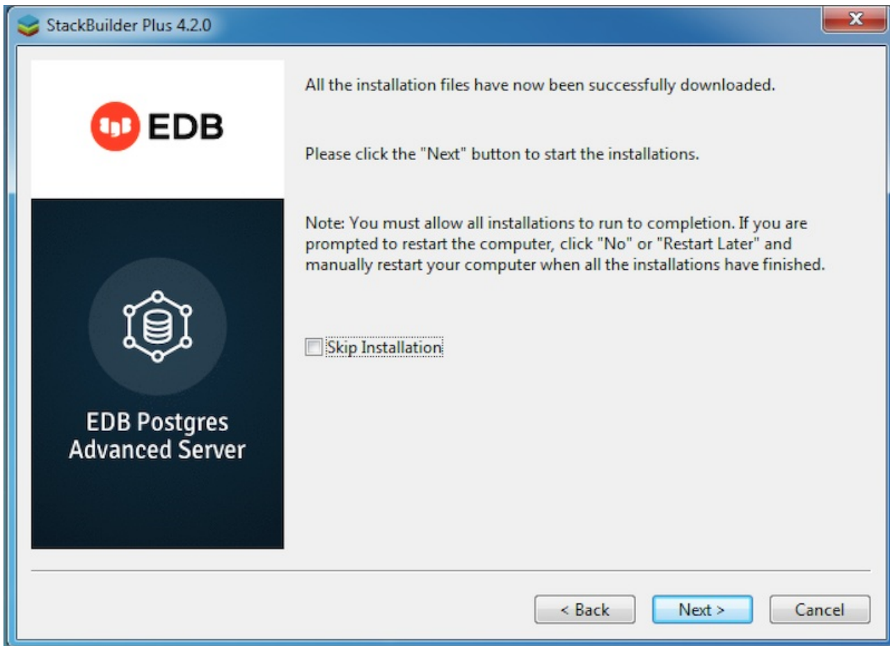
Fig. 2: Installing Slony
