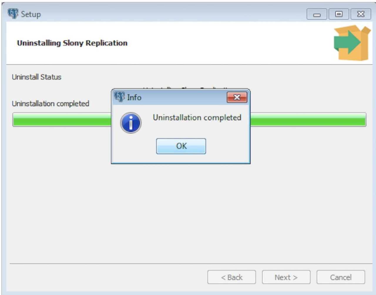
Fig. 2: Uninstallation completes
