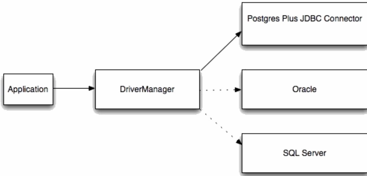
Fig. 3.3: DriverManager/Drivers
