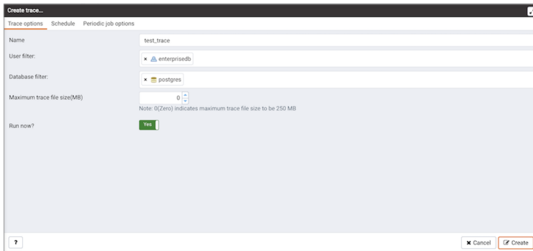
Fig. 2.1: The Trace options tab
