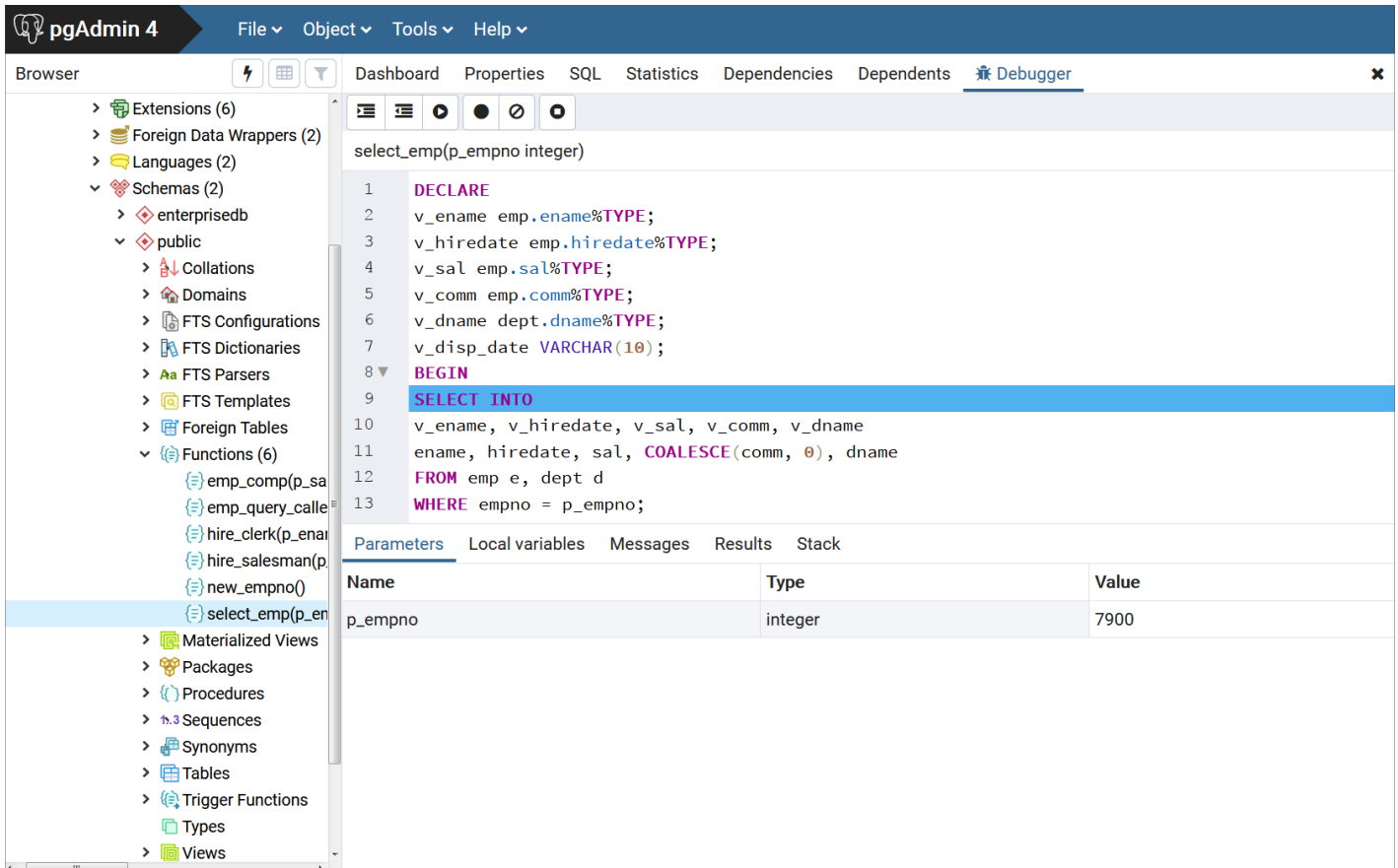
Fig. 19: Program on which a global breakpoint has been set
